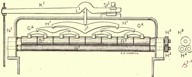
Fig. 33. Elevation Showing Evener Rolls and Levers.
